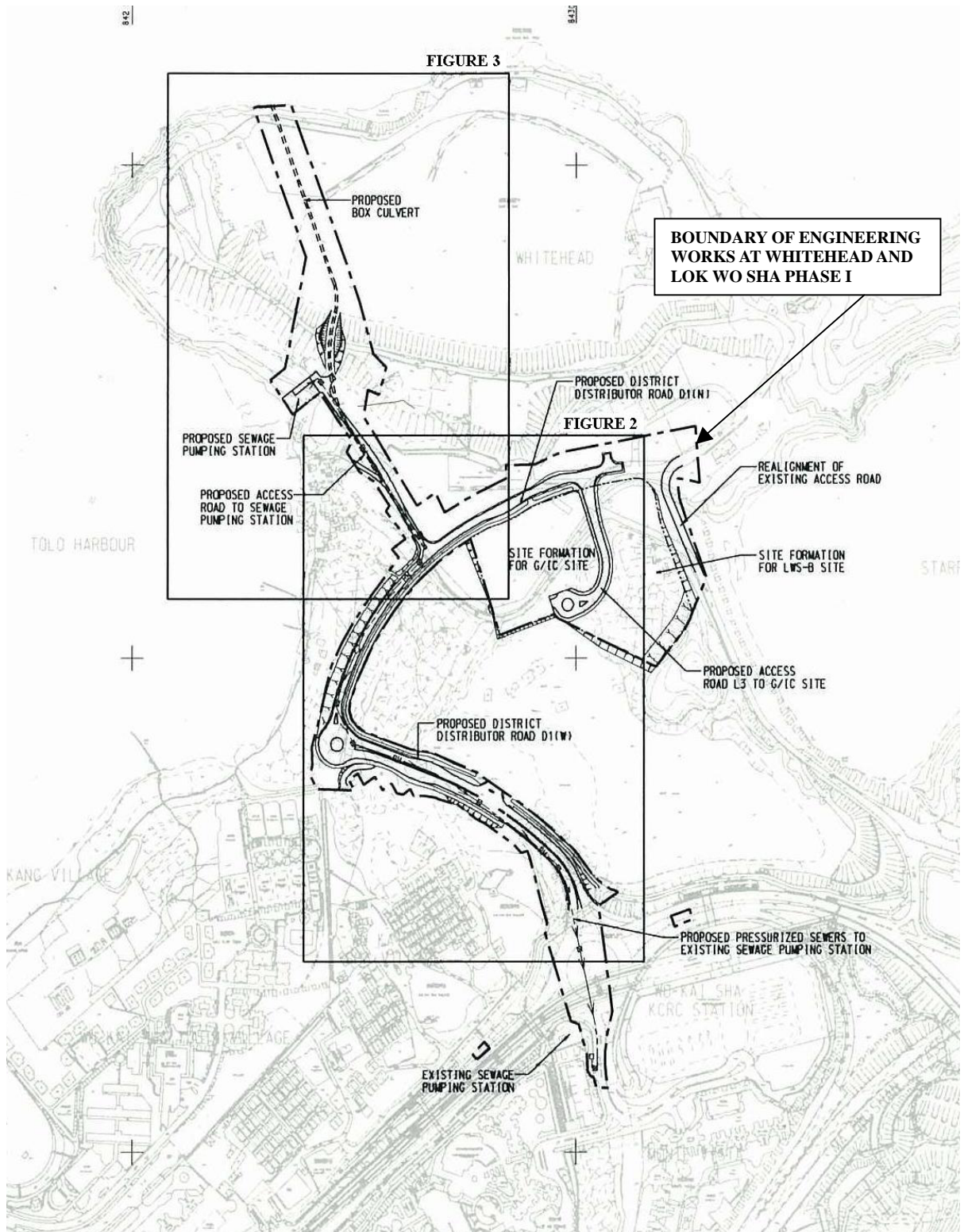
Figure 1: Key Plan
